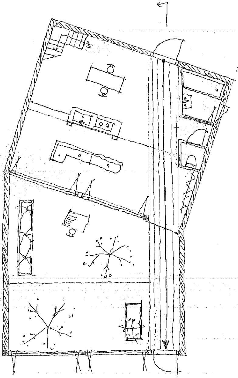
1 F Plan S = 1:100
