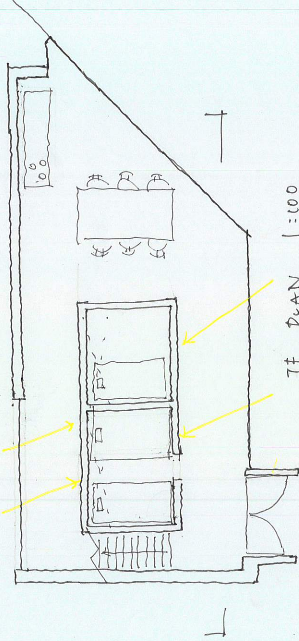
2F PLAN 1:100
