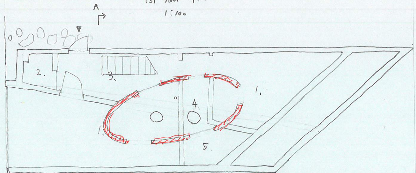
A Ground floor plan 1:100
